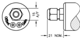
Cable gland, IP67, Option L:
