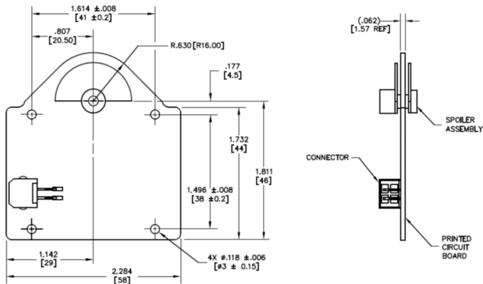
Dimensions are in inch [mm] Minimum area requirement 2 square inches, double sided PCB
